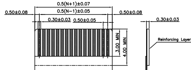
RECOMMENDED FFC DIM
